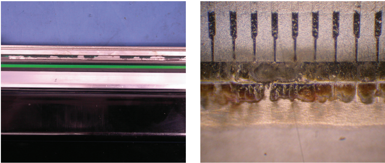
Pictures showing examples of printhead damage that can occur when using non-Zebra ribbons
